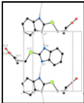
Fig. 2. Partial packing view showing the chain formed by N-H...N hydrogen bondings. H atoms not involved in hydrogen bonds have been omitted for clarity. [Symmetry code: (i) - x+1/2, y+1/2, z ]
